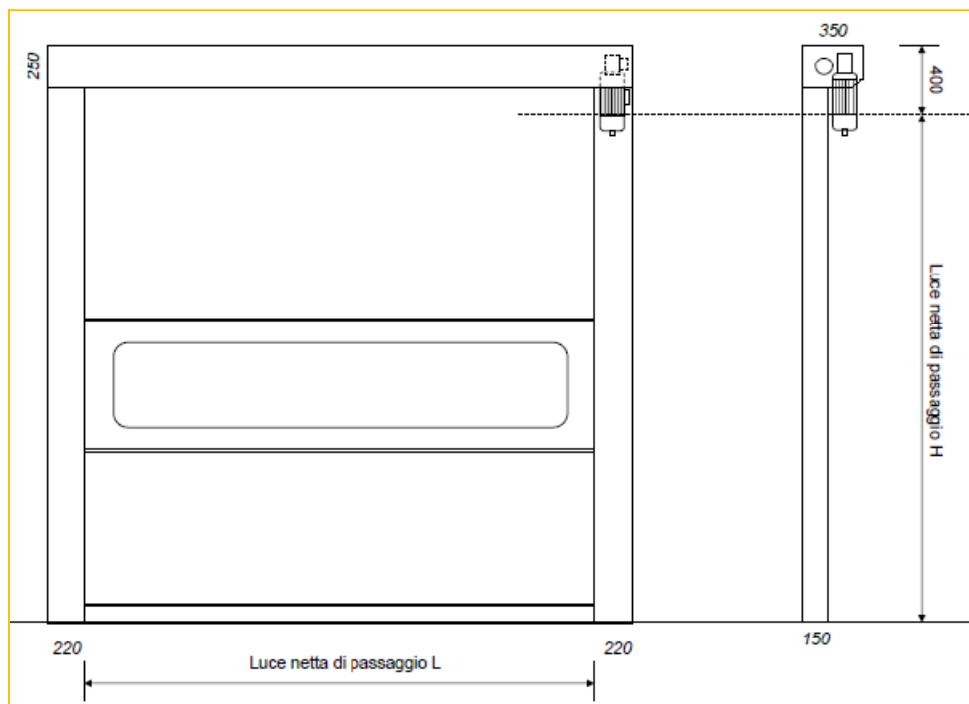
Rolligo FI – Internal front mounting
