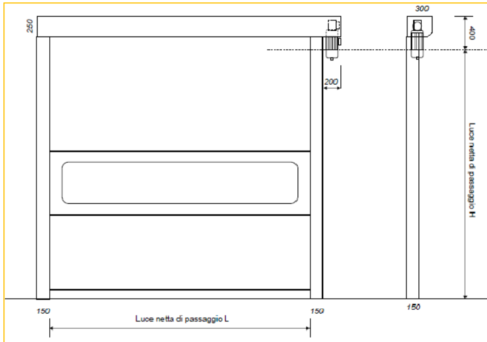
Rolligo L – Side mounting Motor
